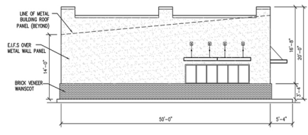
4 SOUTH END ELEVATION 1/8" = 1'-0"
