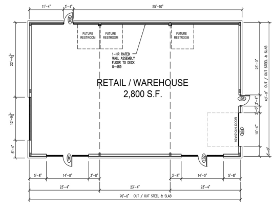
1 RETAIL / WAREHOUSE FLOOR PLAN 1/8" = 1'-0"
