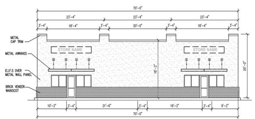
2 FRONT (SOUTH) ELEVATIONS 1/8" = 1'-0"
