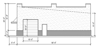
3 NORTH END ELEVATION 1/8" = 1'-0"
